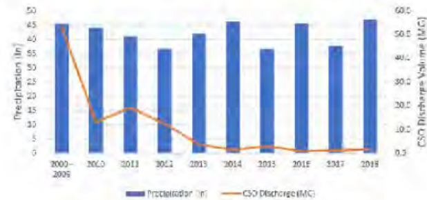
FIGURE 3-6 Auburn Sewer District 2000-2018 Precipitation vs. CSO Discharge
